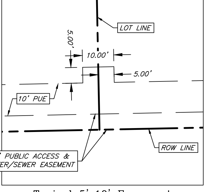
Typical 5'x10' Easement Extension N.T.S.
